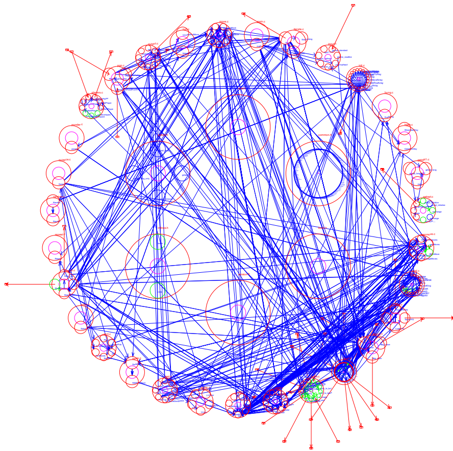
Figure 4: J-Plot Showing Only Calls To Routines
