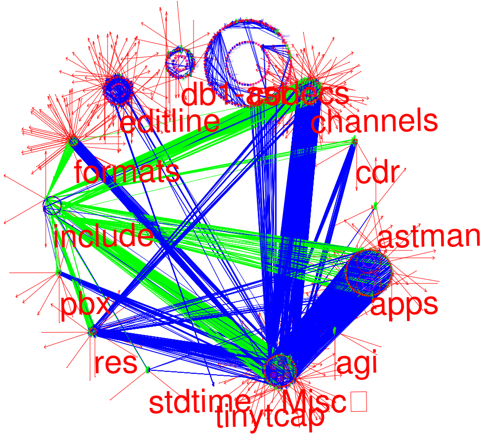
Figure 1: Example J-Plot Showing Only Calls To Modules
